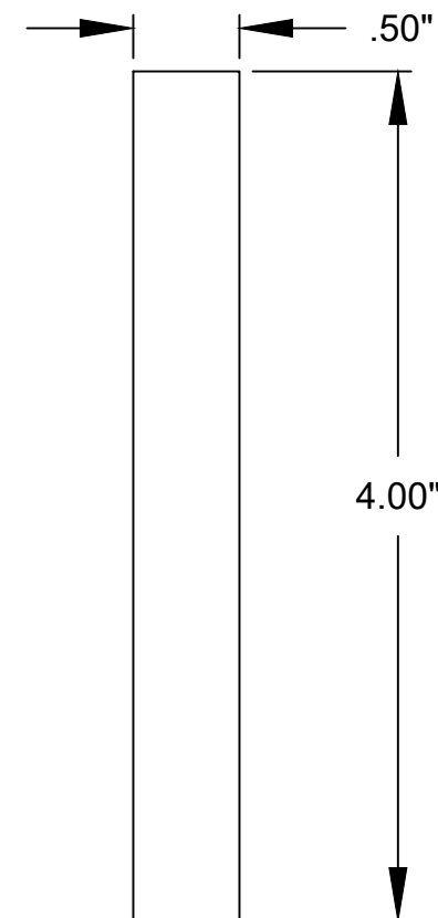
MULLION STIFFENER (6063-T5)
