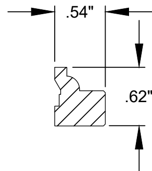
GLAZING BEAD (PINE)
