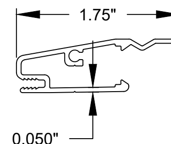
FRAME CLAD (6063-T5)
