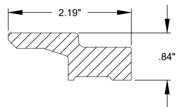
SIDE JAMB COVER (PINE)
